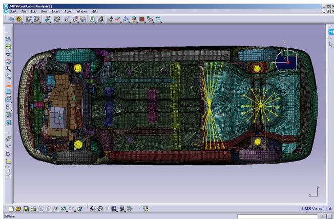
Figure 6: Lumped mass trimming of vehicle.
