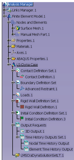
Figure 5: Feature tree of drop test analysis, showing all steps of the process
