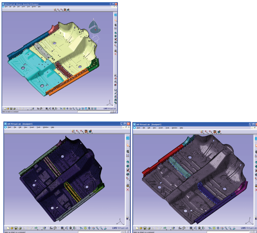
Figure 7: From assembly defined on CAD towards crash and NVH representations
