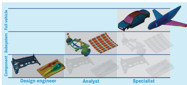
Figure 3: A scalable solution for general finite element analysis
